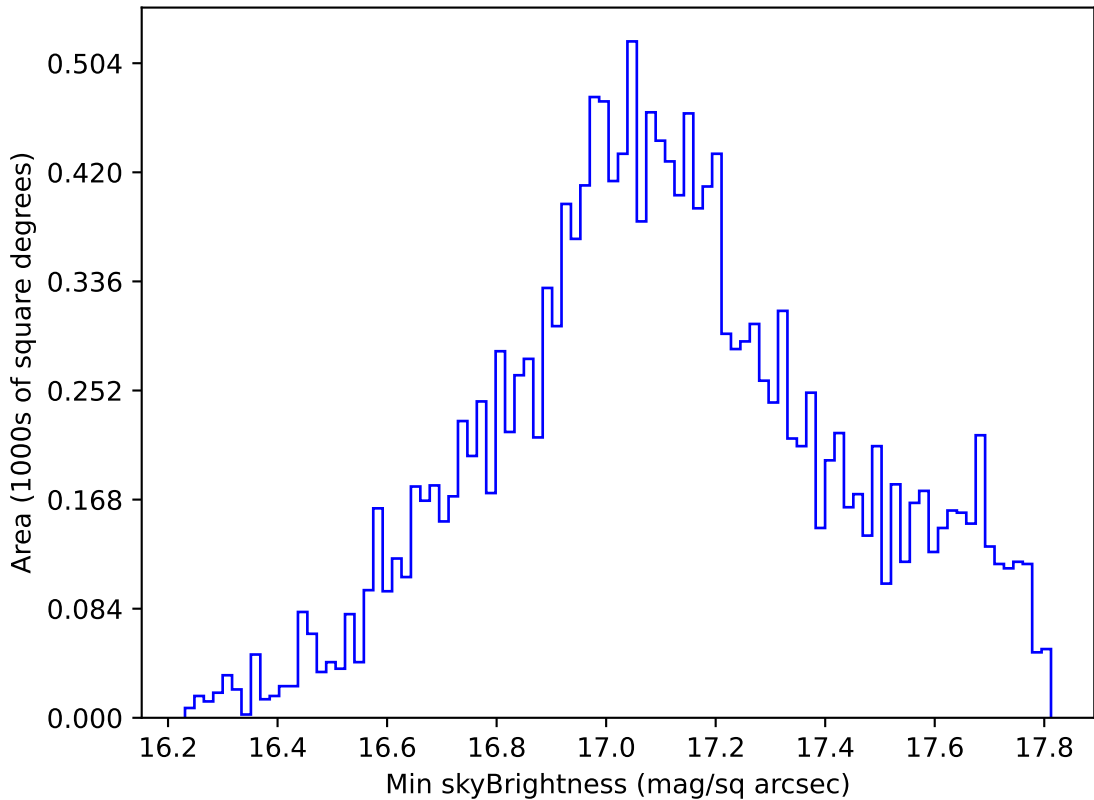
ddf_acor_sf25_lsf40_lsr20_v3.4_10yrs WFD y band: Min skyBrightness
