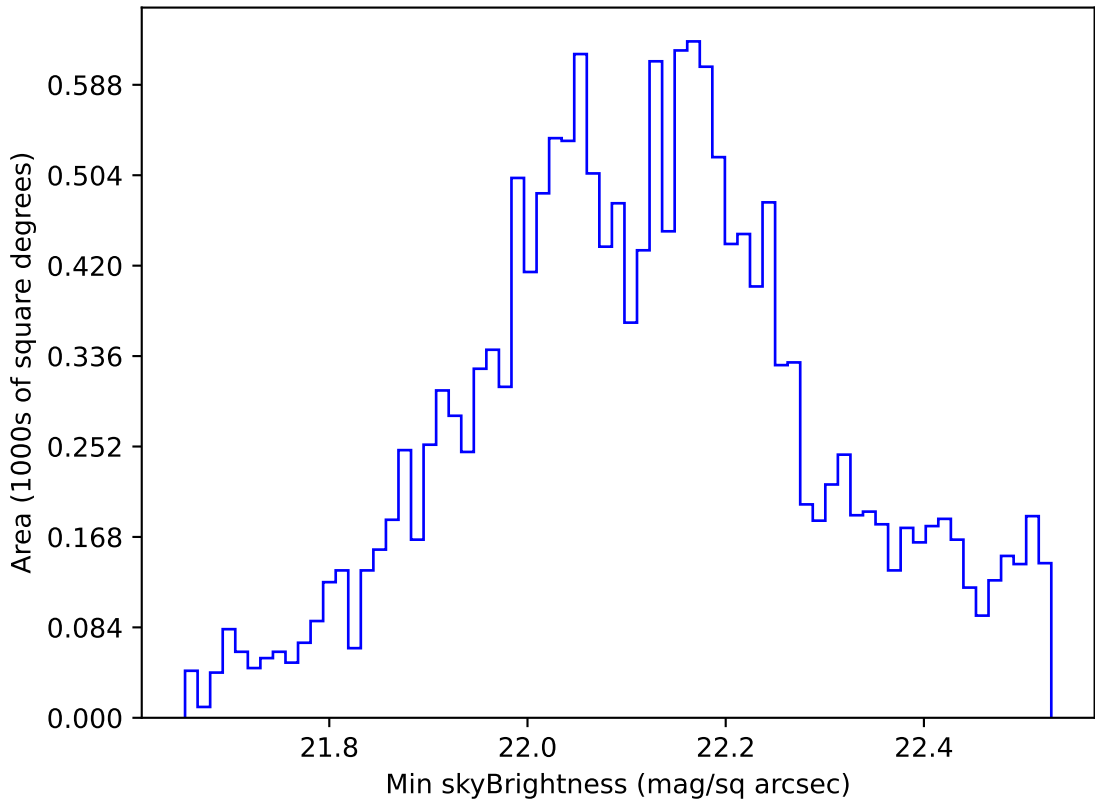
ddf_acor_sf25_lsf40_lsr20_v3.4_10yrs WFD u band: Min skyBrightness
