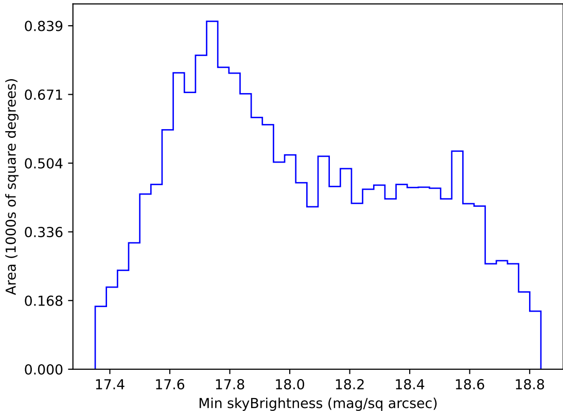
ddf_acor_sf25_lsf40_lsr20_v3.4_10yrs WFD i band: Min skyBrightness
