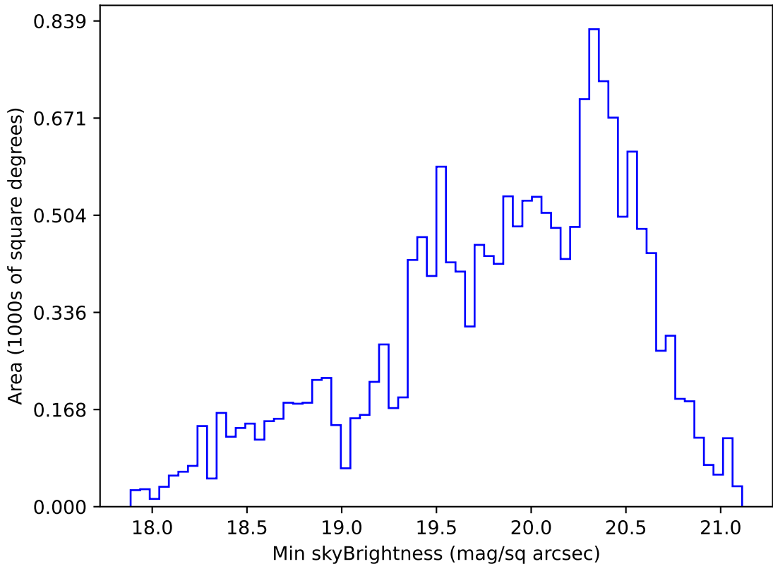
ddf_acor_sf25_lsf40_lsr20_v3.4_10yrs WFD g band: Min skyBrightness
