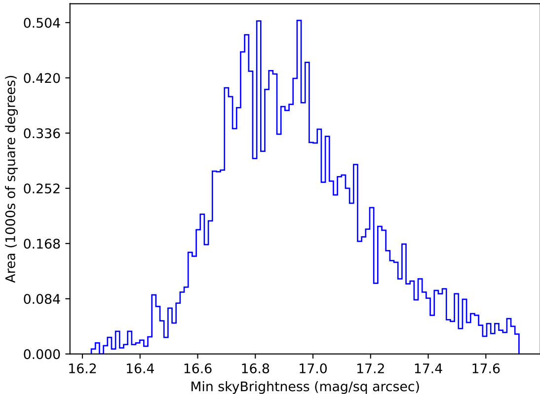
ddf_acor_sf25_lsf40_lsr20_v3.4_10yrs WFD all bands: Min skyBrightness
