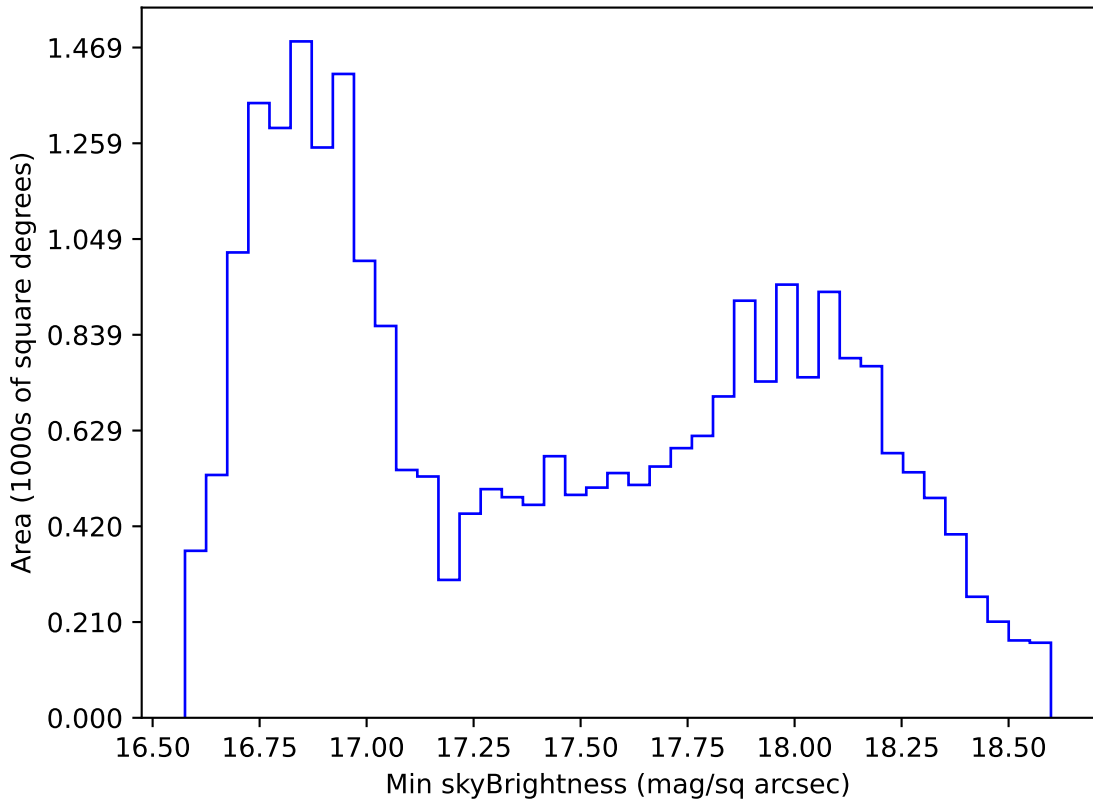
ddf_acor_sf25_lsf40_lsr20_v3.4_10yrs All sky z band: Min skyBrightness
