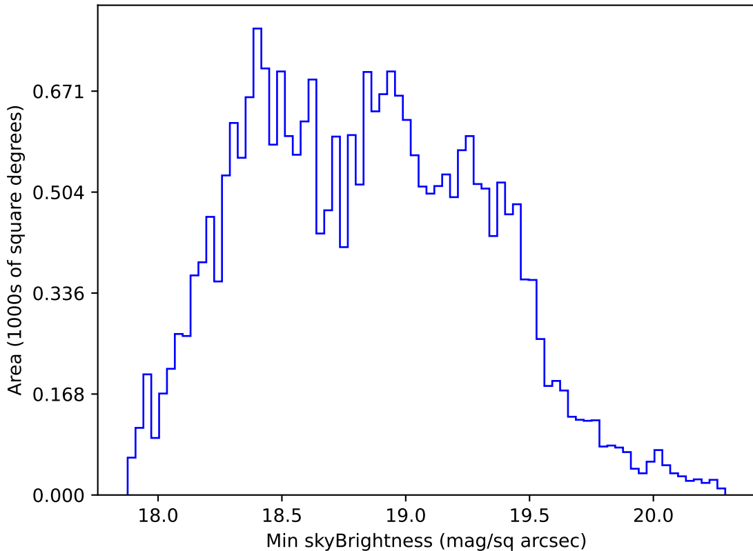
ddf_acor_sf25_lsf40_lsr20_v3.4_10yrs All sky r band: Min skyBrightness
