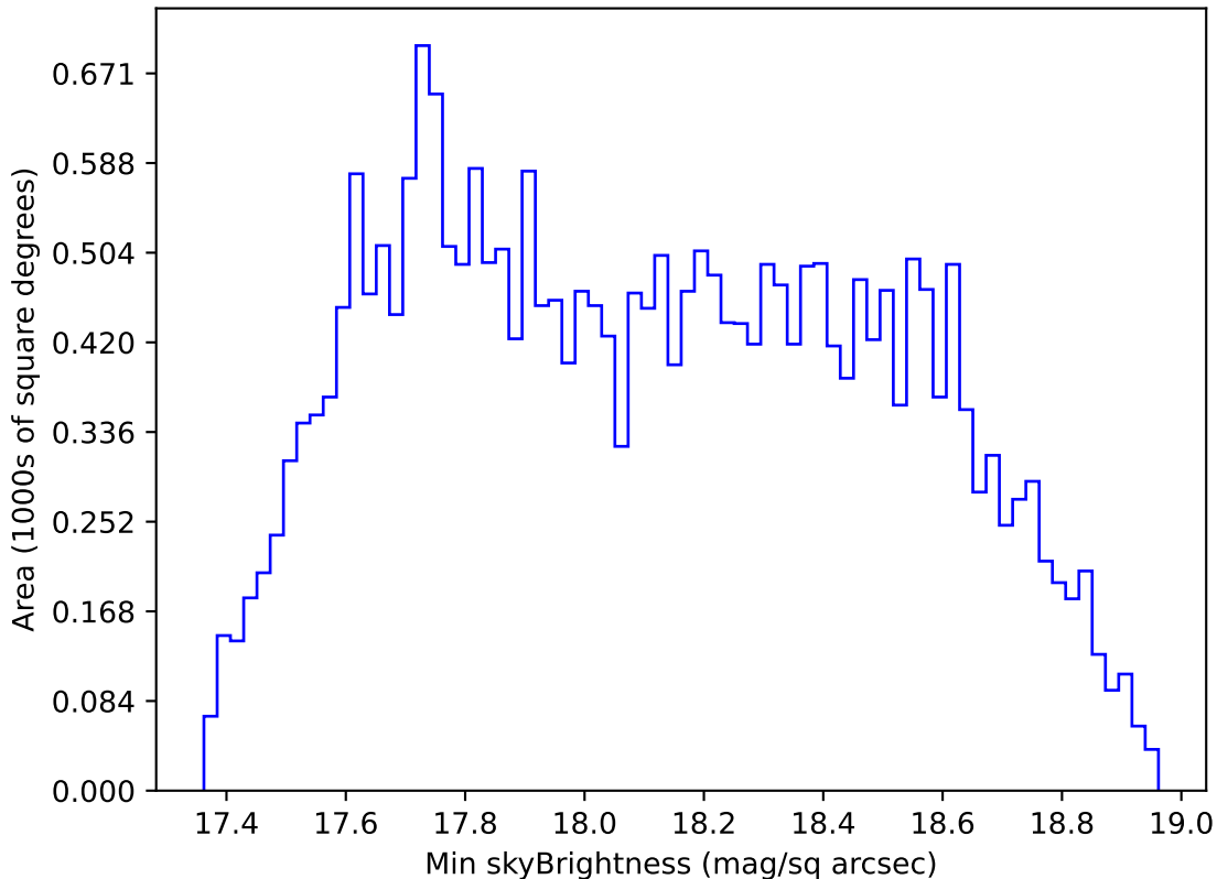
ddf_acor_sf25_lsf40_lsr20_v3.4_10yrs All sky i band: Min skyBrightness
