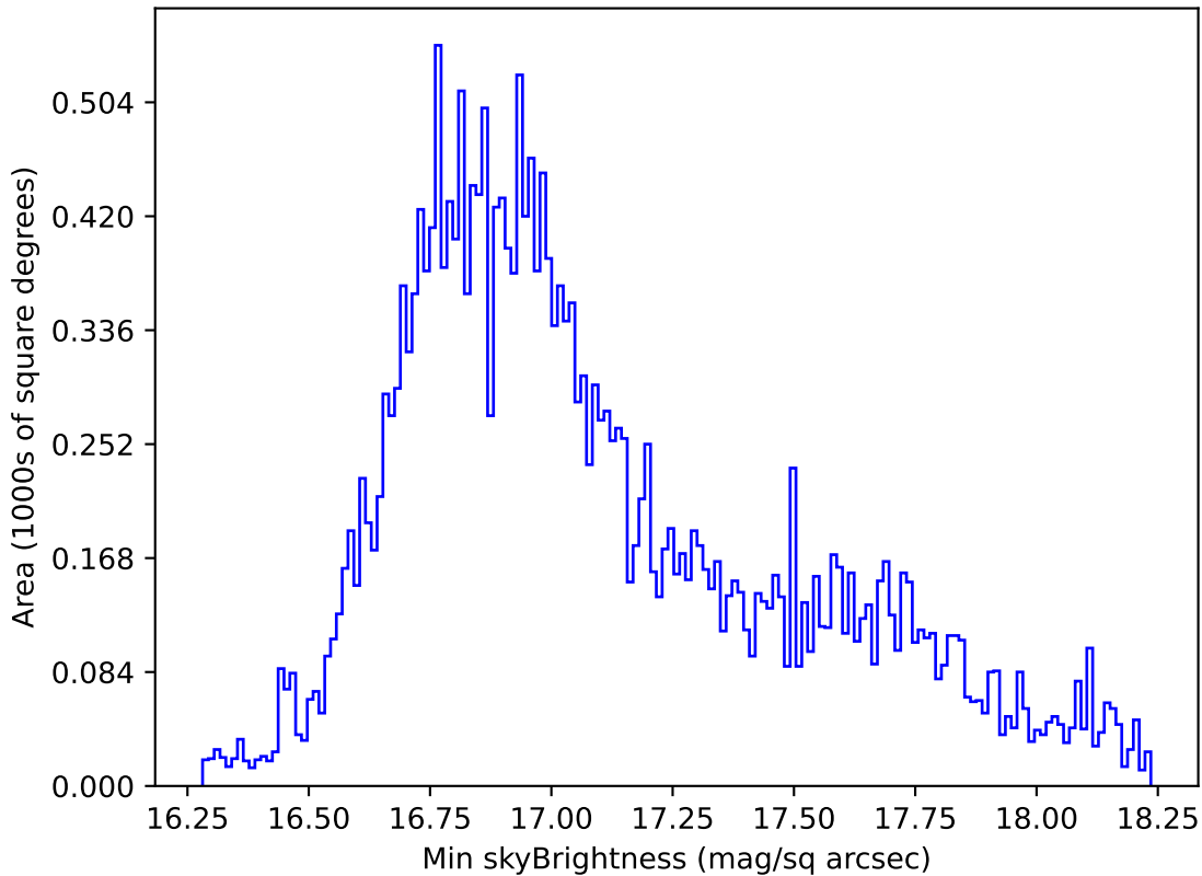
ddf_acor_sf25_lsf40_lsr20_v3.4_10yrs All sky all bands: Min skyBrightness
