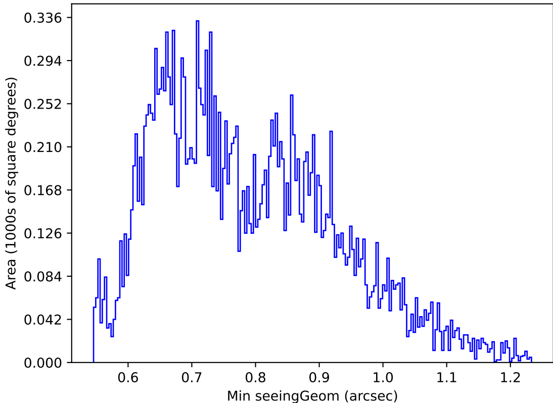
ddf_acor_sf25_ls40_lsr20_v3.4_10yrs Yr 1 u band: Min seeingGeom
