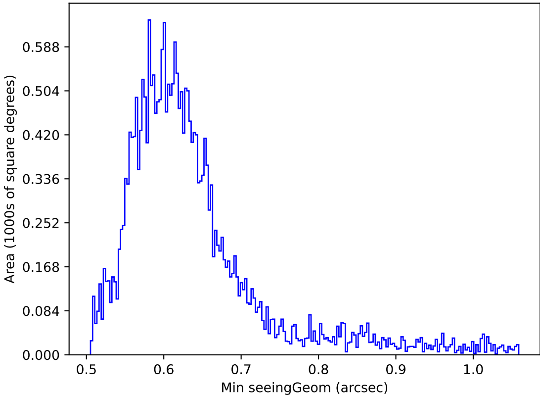
ddf_acor_sf25_lsf40_lsr20_v3.4_10yrs Yr 1 r band: Min seeingGeom
