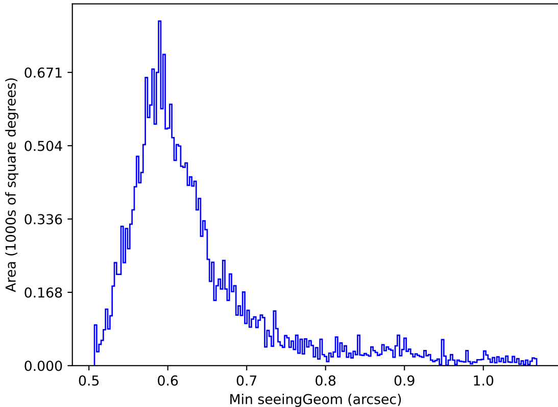
ddf_acor_sf25_lsf40_lsr20_v3.4_10yrs Yr 1 i band: Min seeingGeom
