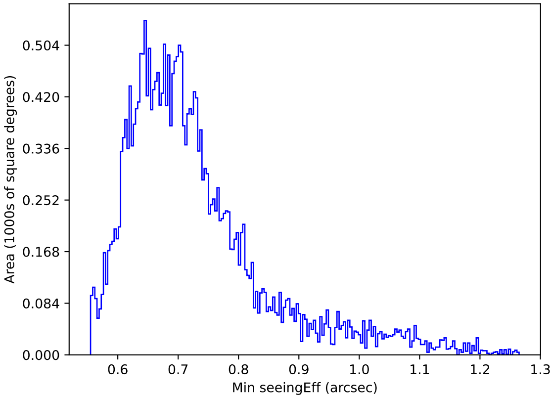
ddf_acor_sf25_lsf40_lsr20_v3.4_10yrs Yr 1 z band: Min seeingEff
