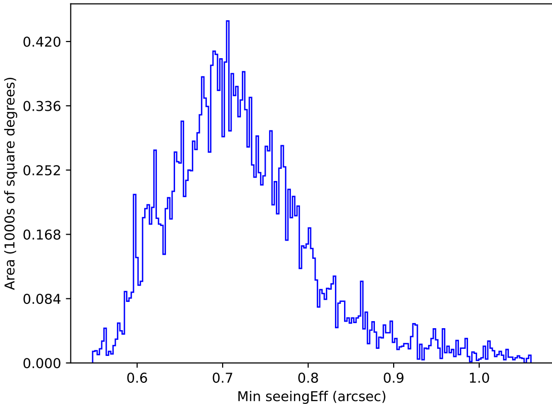
ddf_acor_sf25_lsf40_lsr20_v3.4_10yrs Yr 1 y band: Min seeingEff
