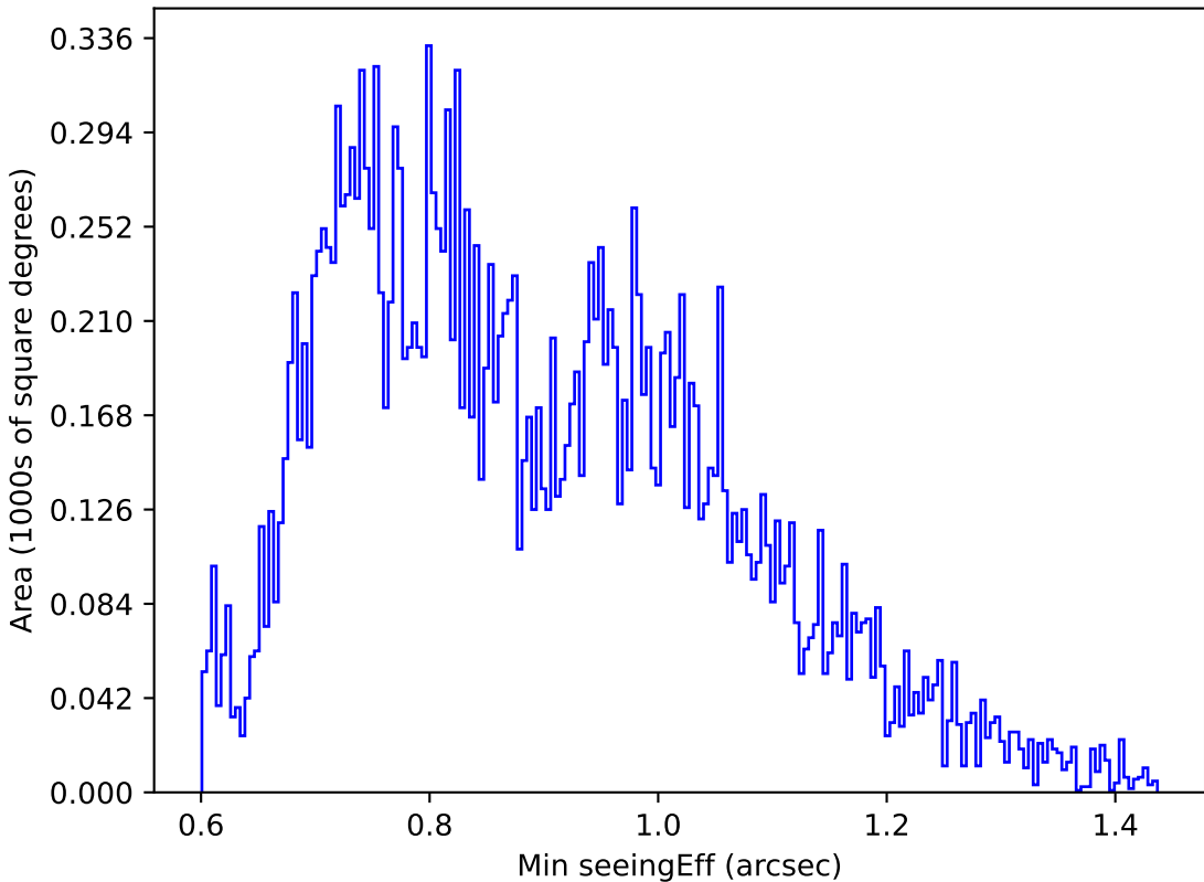
ddf_acor_sf25_lsf40_lsr20_v3.4_10yrs Yr 1 u band: Min seeingEff
