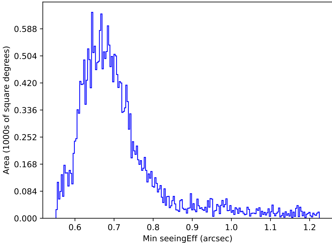
ddf_acor_sf25_Isf40_Isr20_v3.4_10yrs Yr 1 r band: Min seeingEff
