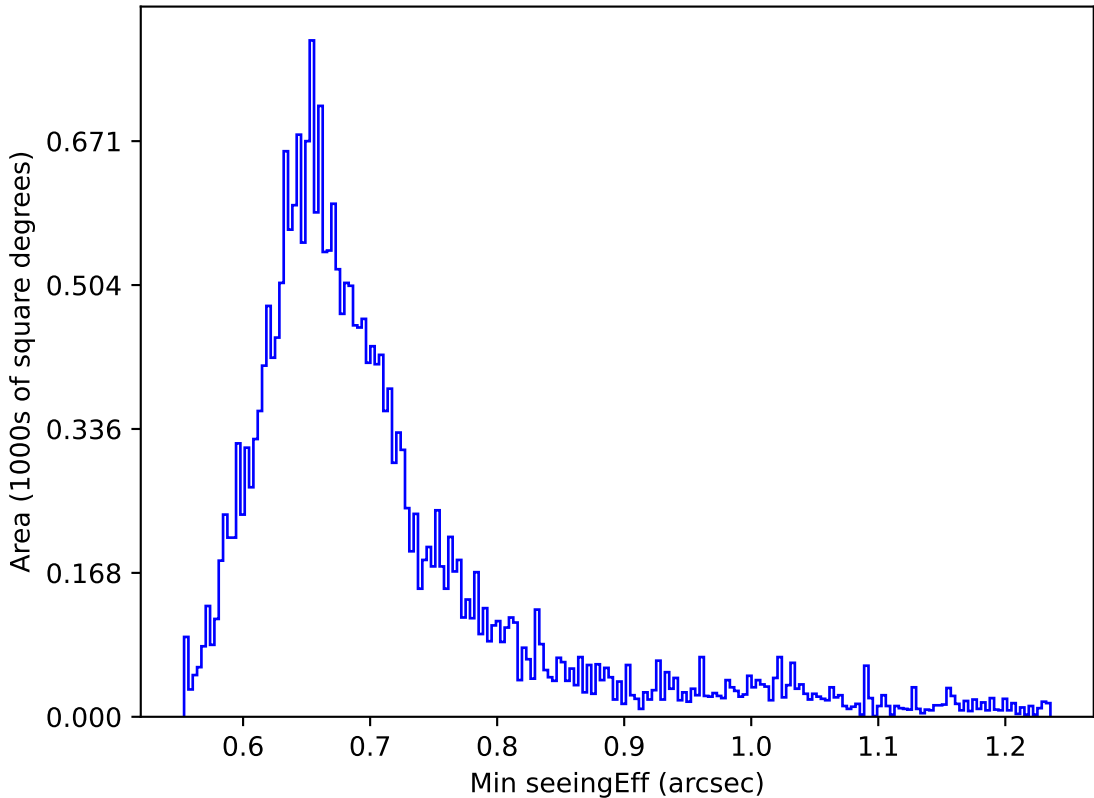
ddf_acor_sf25_lsf40_lsr20_v3.4_10yrs Yr 1 i band: Min seeingEff
