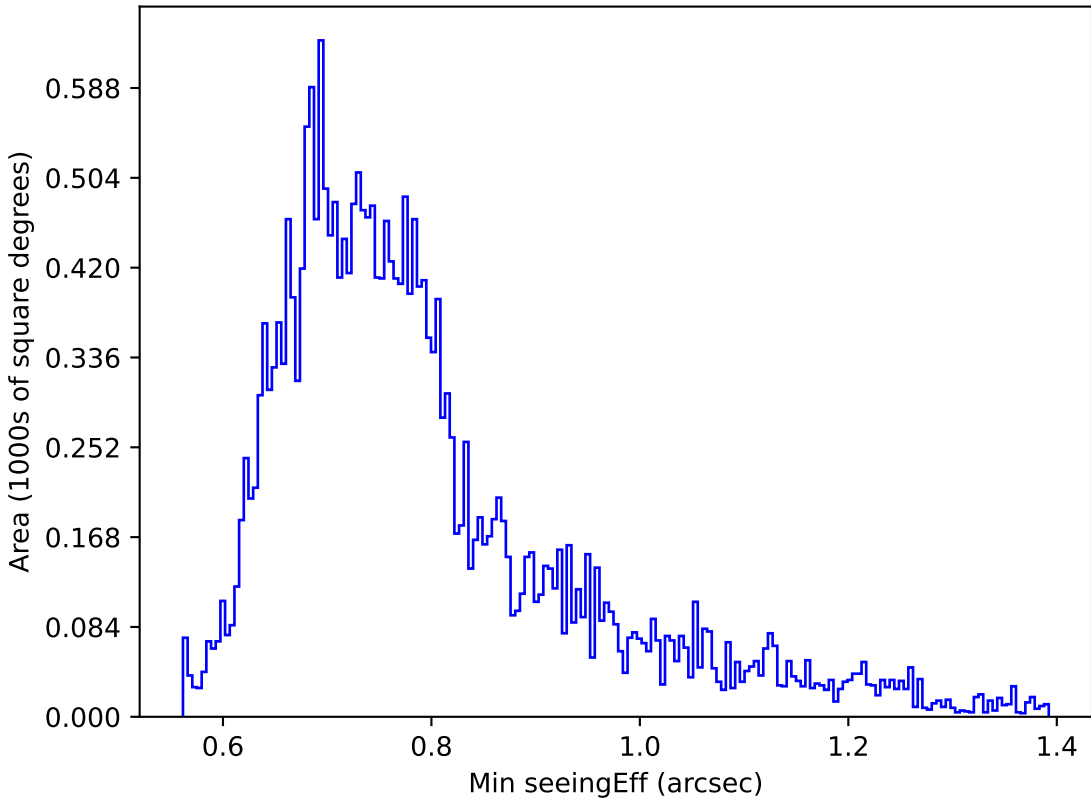
ddf_acor_sf25_lsf40_lsr20_v3.4_10yrs Yr 1 g band: Min seeingEff
