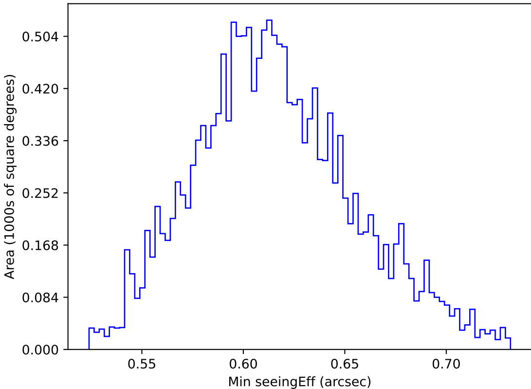
ddf_acor_sf25_lsf40_lsr20_v3.4_10yrs WFD z band: Min seeingEff
