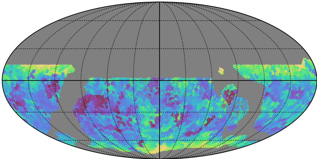
ddf_acor_sf25_lsf40_lsr20_v3.4_10yrs WFD y band: Min seeingEff
