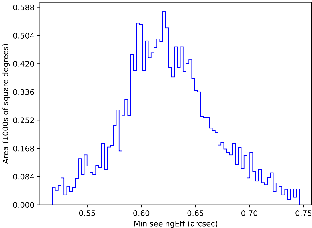
ddf_acor_sf25_lsf40_lsr20_v3.4_10yrs WFD y band: Min seeingEff
