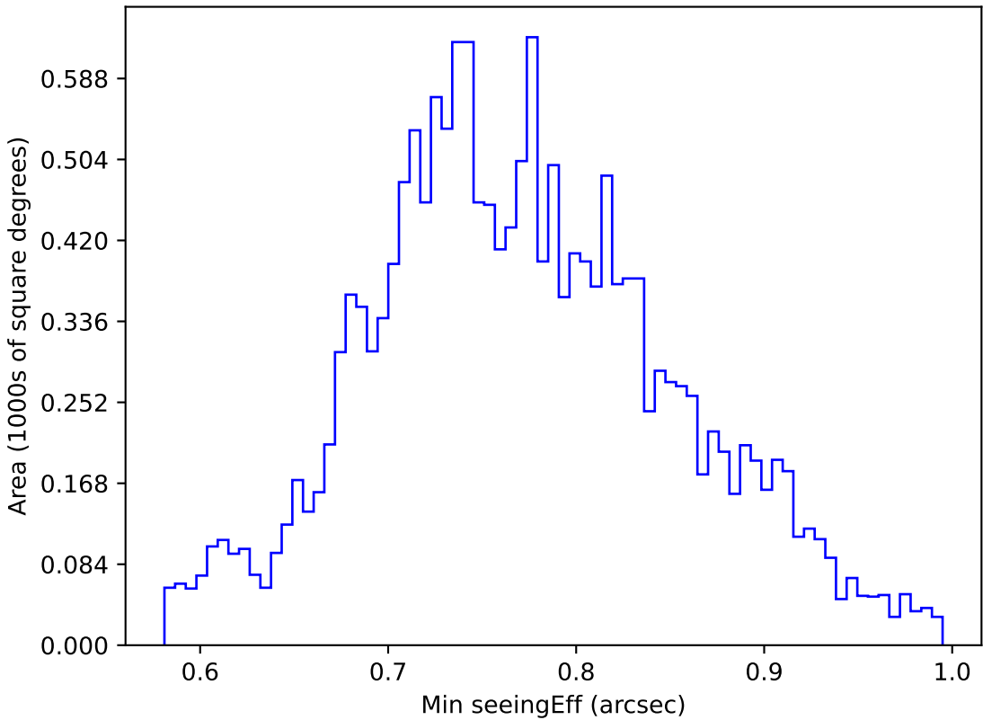
ddf_acor_sf25_lsf40_lsr20_v3.4_10yrs WFD u band: Min seeingEff
