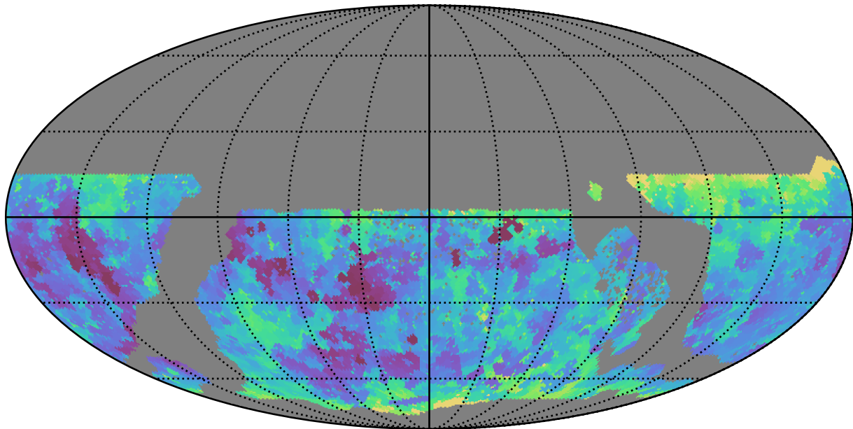
ddf_acor_sf25_lsf40_lsr20_v3.4_10yrs WFD g band: Min seeingEff
