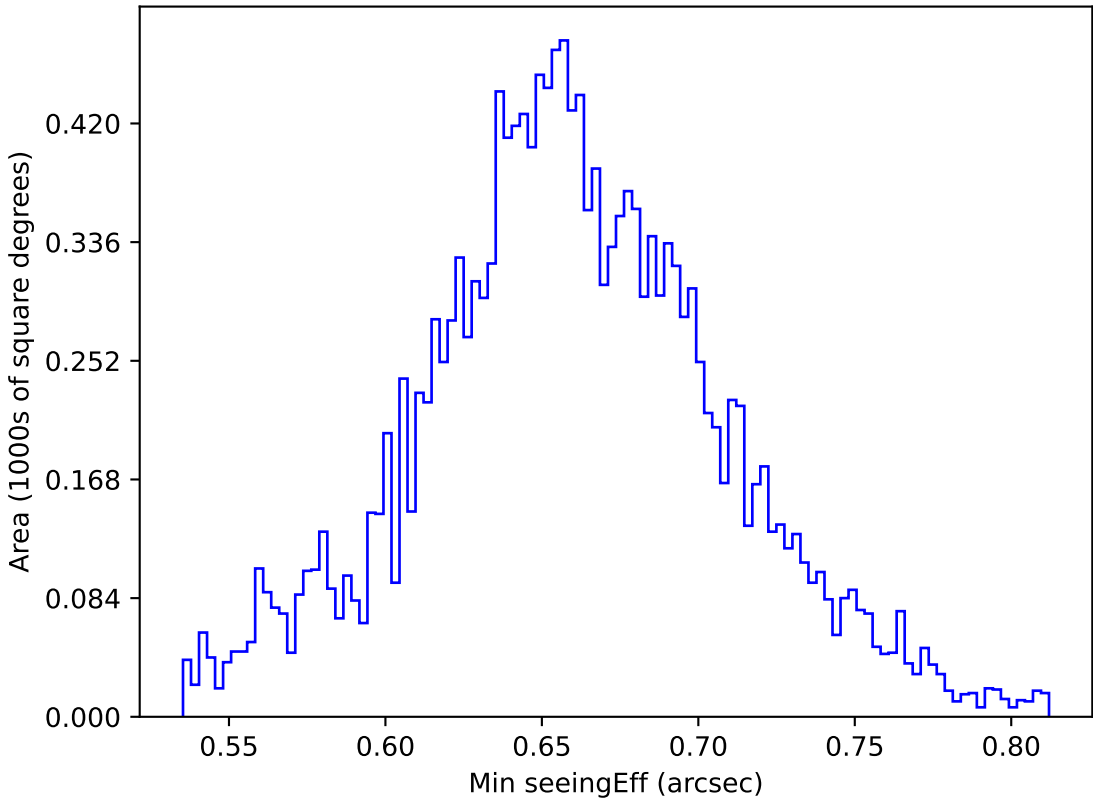
ddf_acor_sf25_lsf40_lsr20_v3.4_10yrs WFD g band: Min seeingEff
