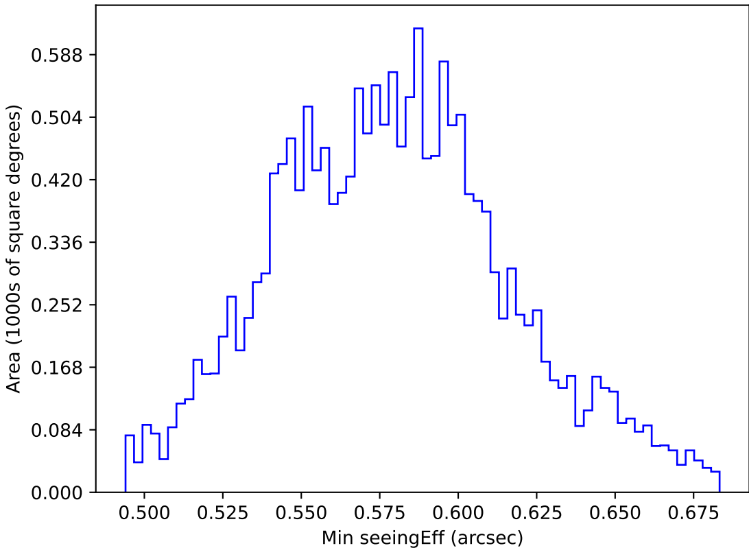
ddf_acor_sf25_lsf40_lsr20_v3.4_10yrs WFD all bands: Min seeingEff
