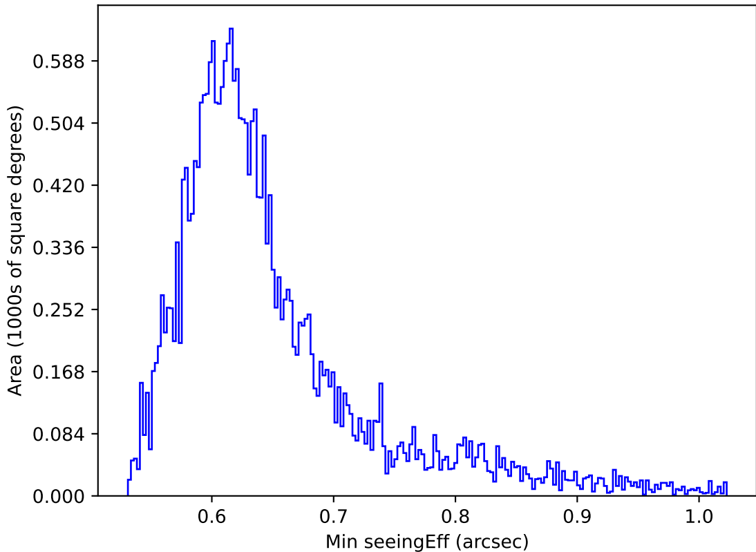
ddf_acor_sf25_lsf40_lsr20_v3.4_10yrs All sky z band: Min seeingEff
