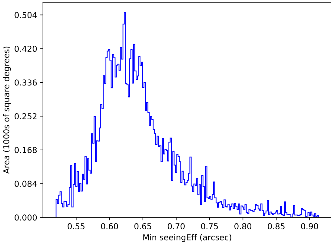
ddf_acor_sf25_lsf40_lsr20_v3.4_10yrs All sky y band: Min seeingEff
