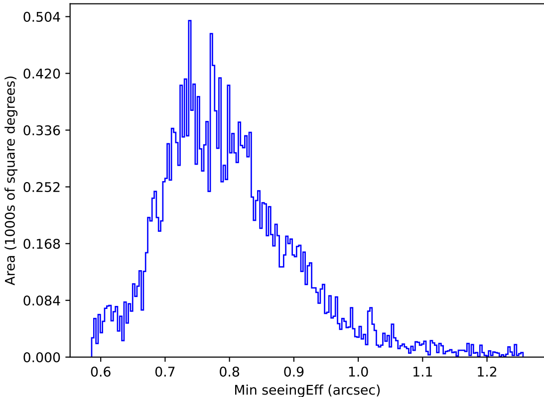
ddf_acor_sf25_lsf40_lsr20_v3.4_10yrs All sky u band: Min seeingEff
