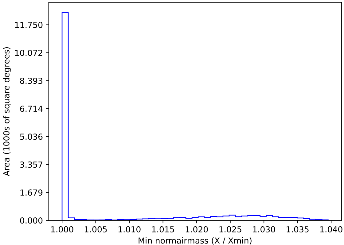
ddf_acor_sf25_lsf40_lsr20_v3.4_10yrs WFD y band: Min normairmass
