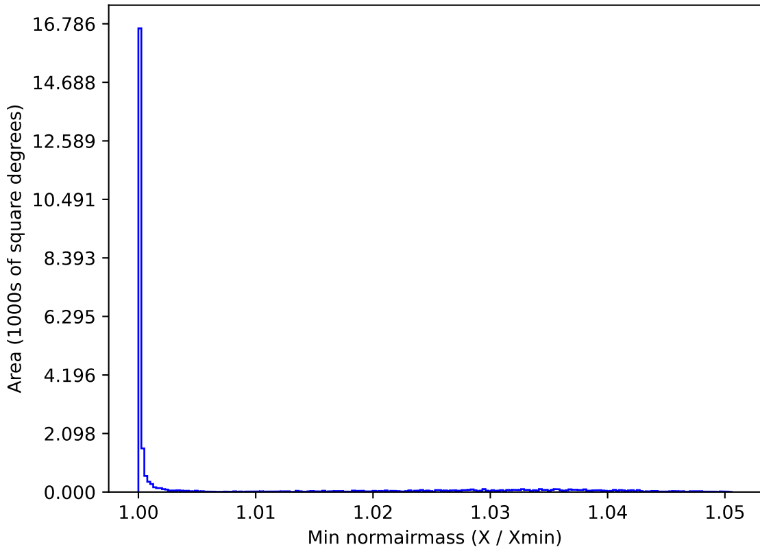
ddf_acor_sf25_lsf40_lsr20_v3.4_10yrs All sky g band: Min normairmass
