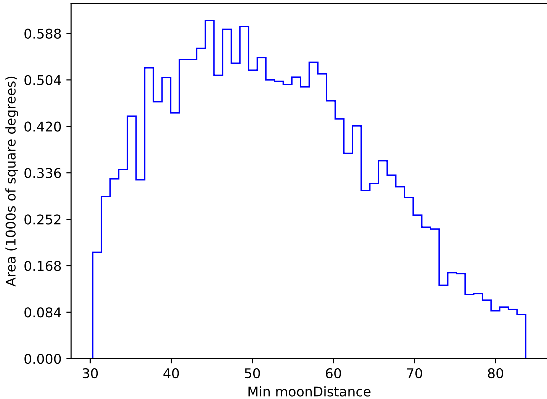
ddf_acor_sf25_lsf40_lsr20_v3.4_10yrs WFD u band: Min moonDistance
