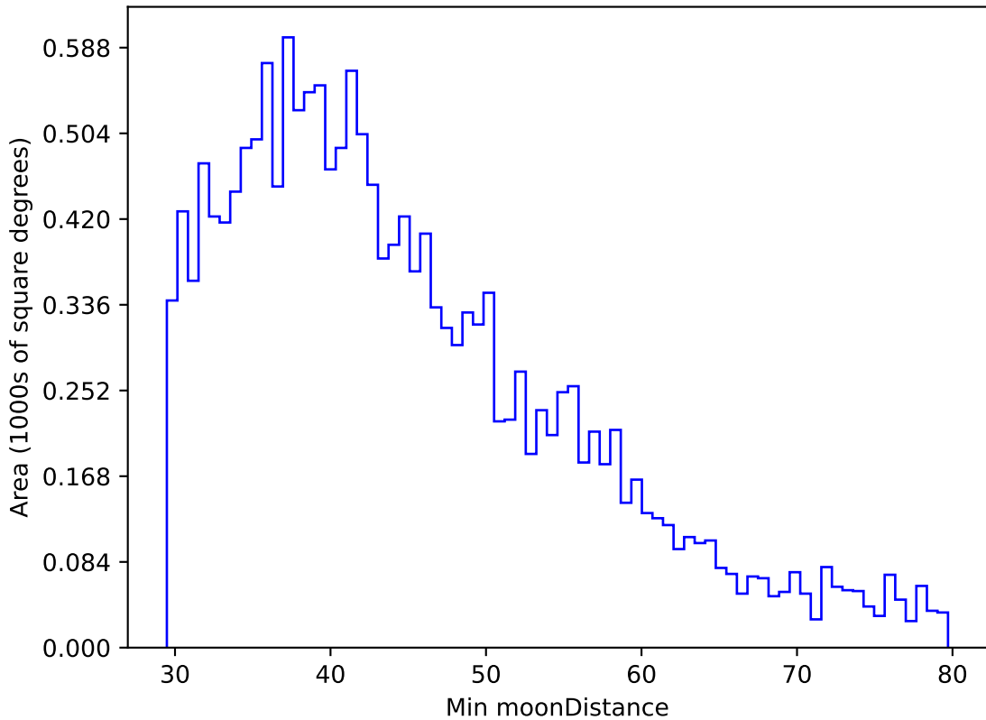
ddf_acor_sf25_lsf40_lsr20_v3.4_10yrs WFD g band: Min moonDistance
