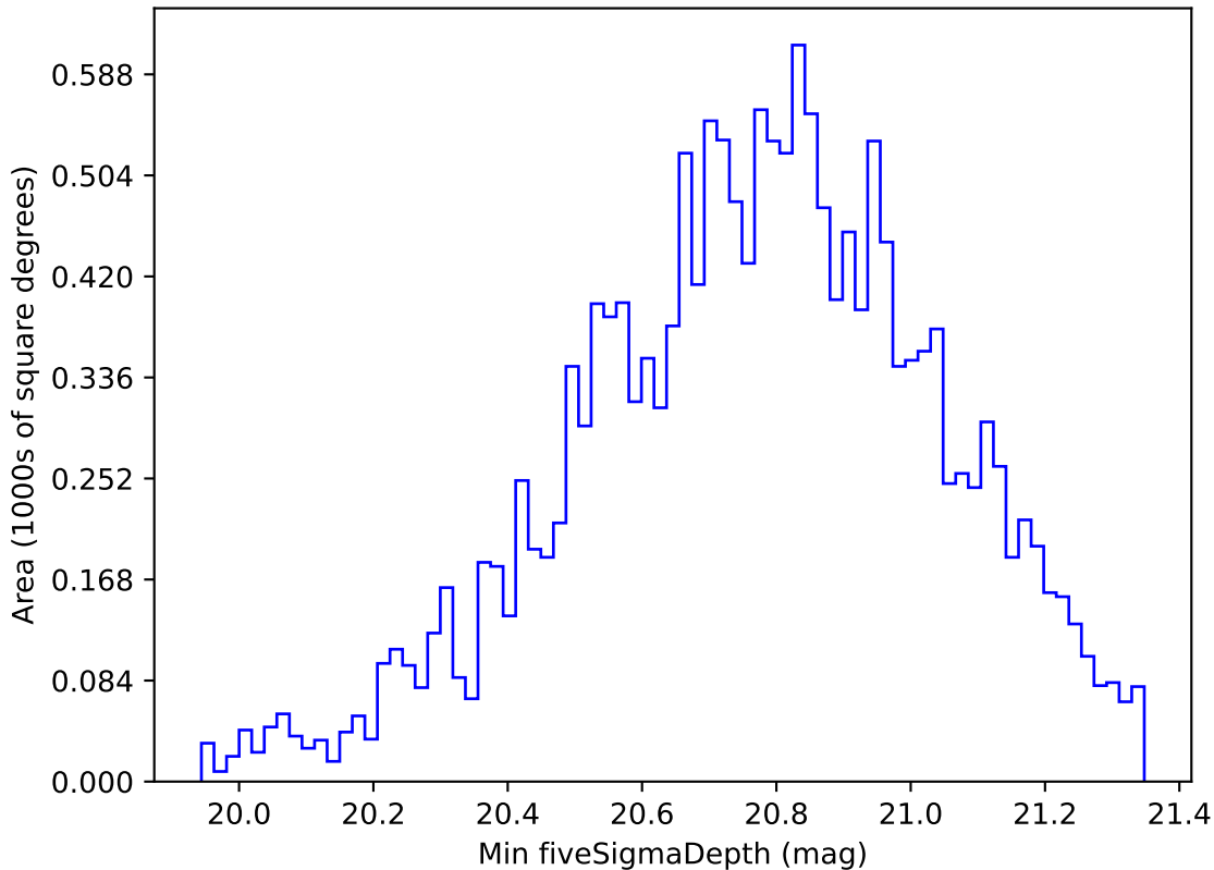
ddf_acor_sf25_lsf40_lsr20_v3.4_10yrs WFD all bands: Min fiveSigmaDepth
