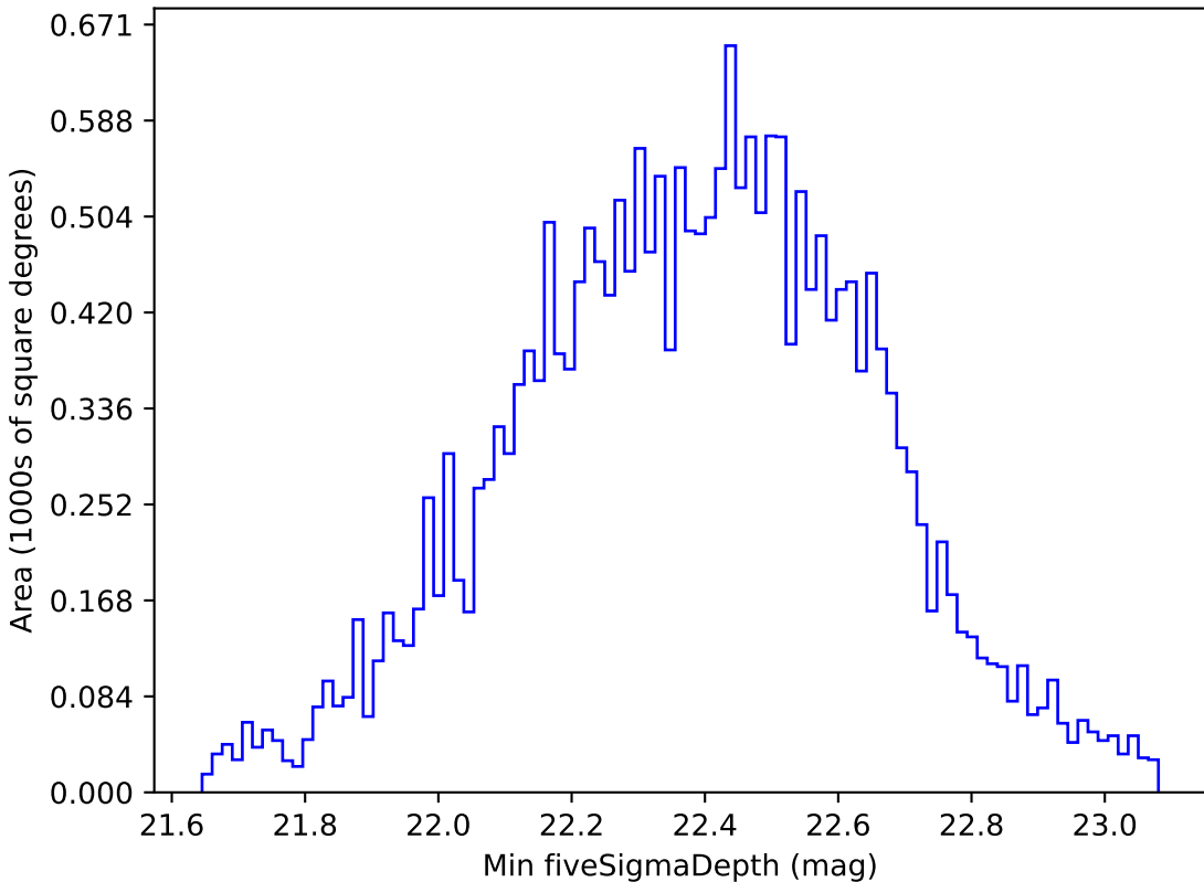
ddf_acor_sf25_lsf40_lsr20_v3.4_10yrs All sky u band: Min fiveSigmaDepth
