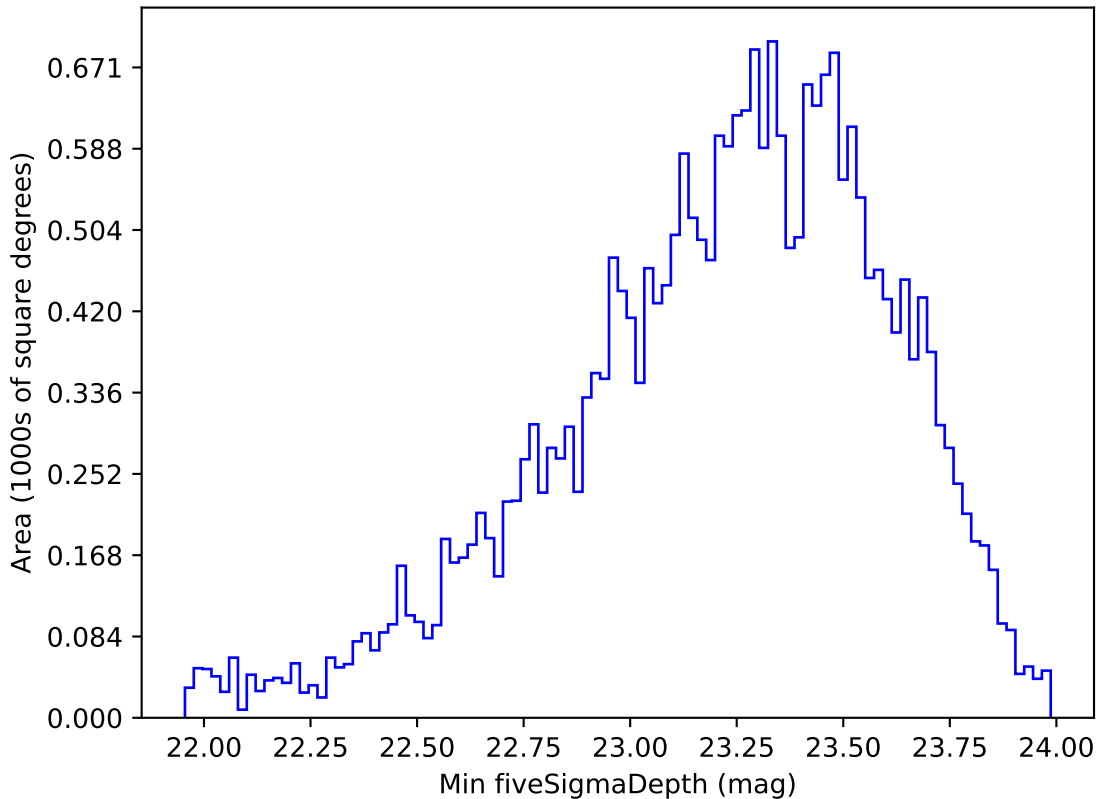
ddf_acor_sf25_lsf40_lsr20_v3.4_10yrs All sky g band: Min fiveSigmaDepth
