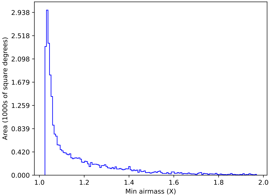
ddf_acor_sf25_lsf40_lsr20_v3.4_10yrs Yr 1 r band: Min airmass
