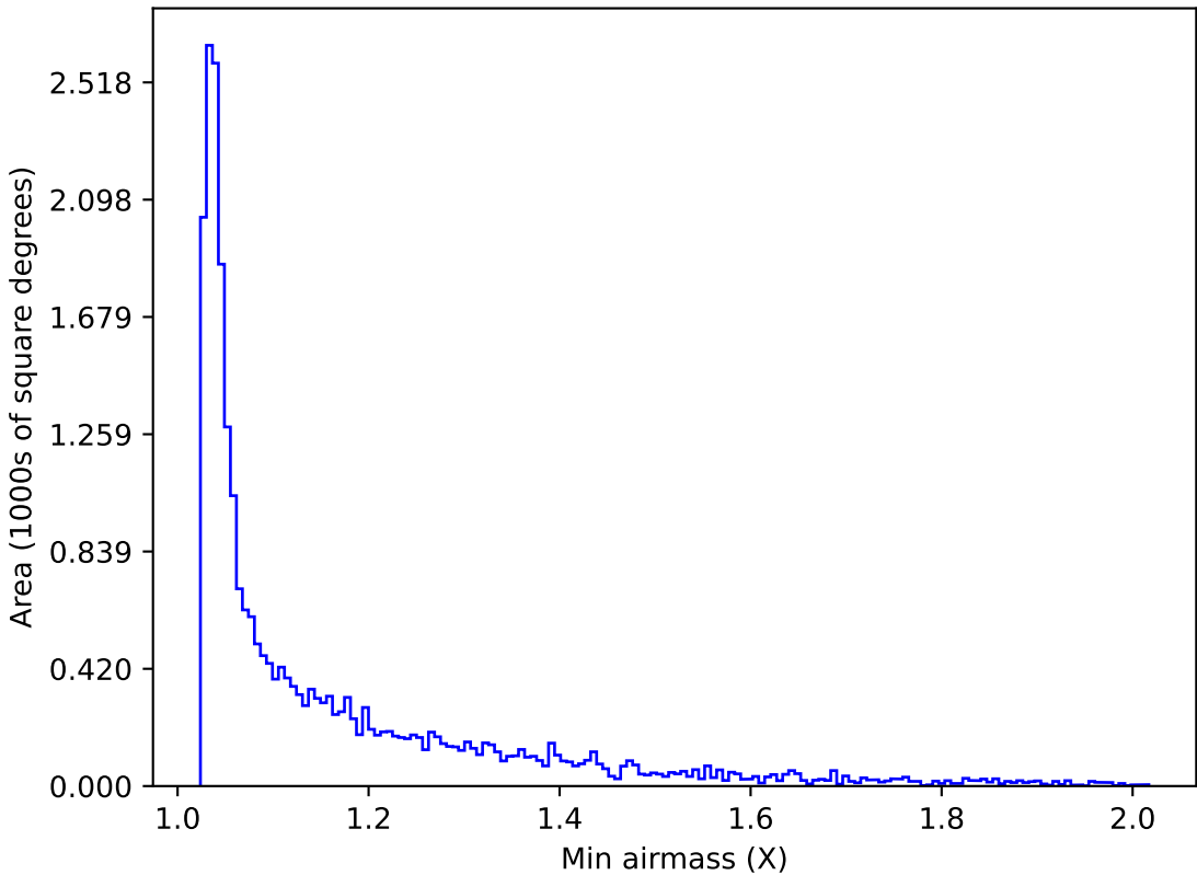
ddf_acor_sf25_lsf40_lsr20_v3.4_10yrs Yr 1 i band: Min airmass
