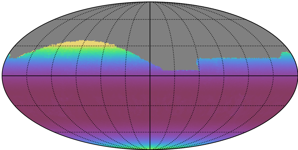
ddf_acor_sf25_lsf40_lsr20_v3.4_10yrs Yr 1 all bands: Min airmass
