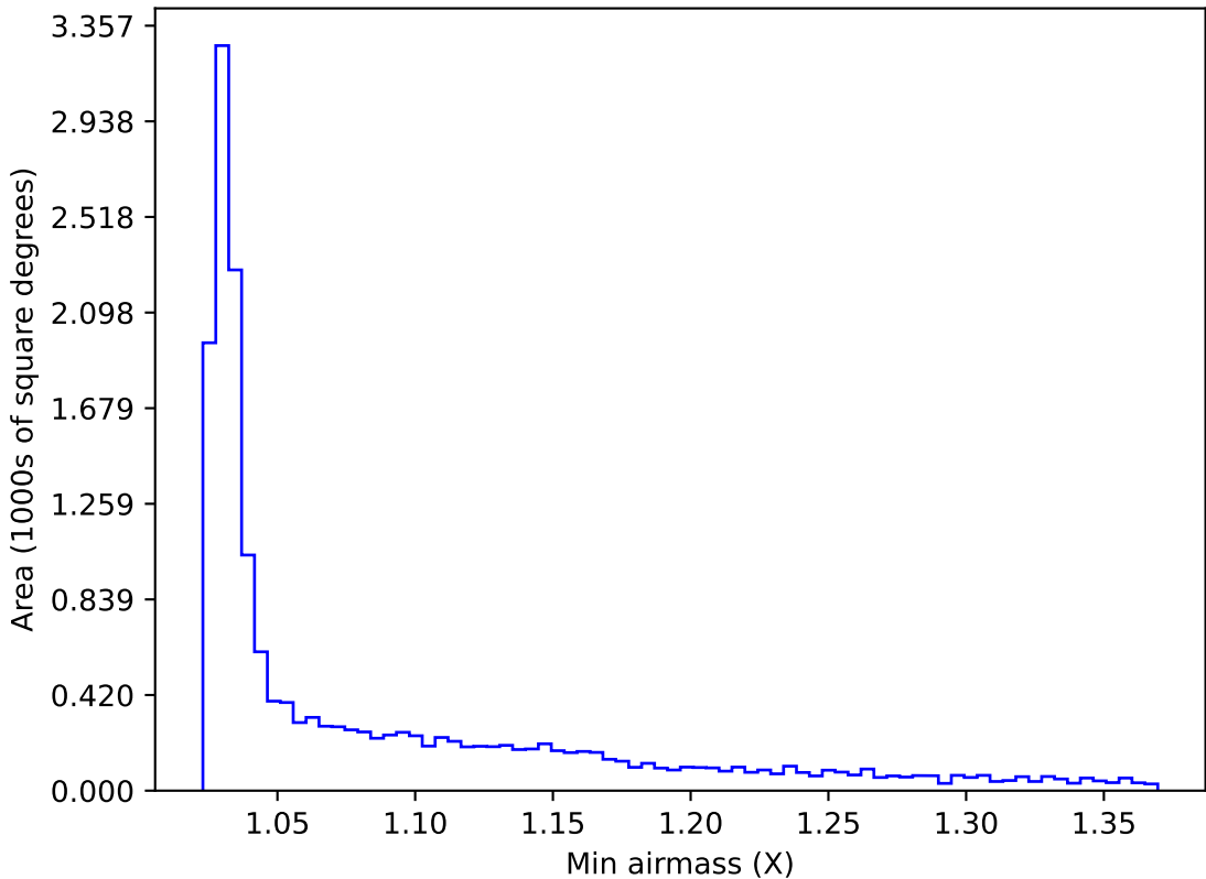
ddf_acor_sf25_lsf40_lsr20_v3.4_10yrs WFD y band: Min airmass
