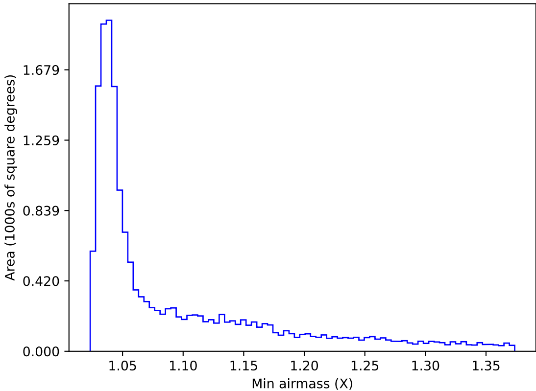
ddf_acor_sf25_lsf40_lsr20_v3.4_10yrs WFD u band: Min airmass
