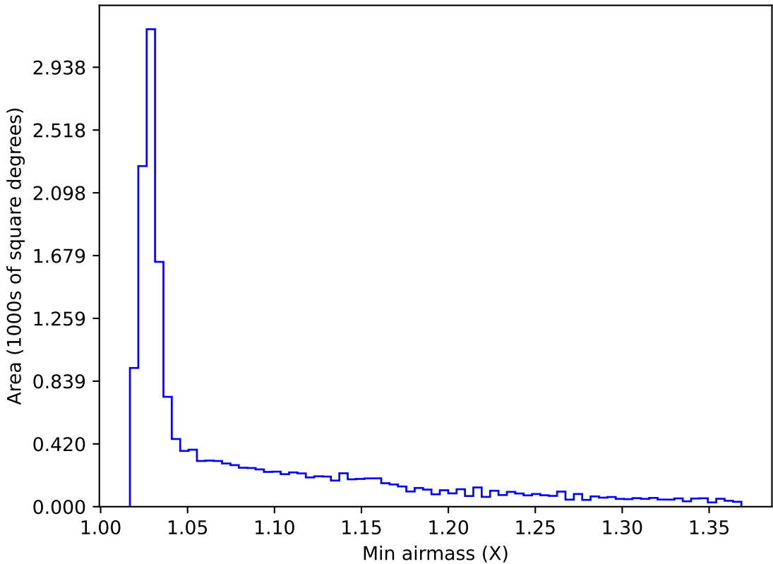
ddf_acor_sf25_lsf40_lsr20_v3.4_10yrs WFD r band: Min airmass
