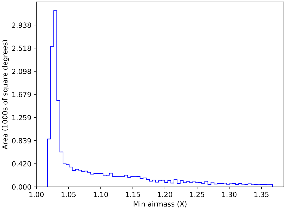
ddf_acor_sf25_lsf40_lsr20_v3.4_10yrs WFD i band: Min airmass
