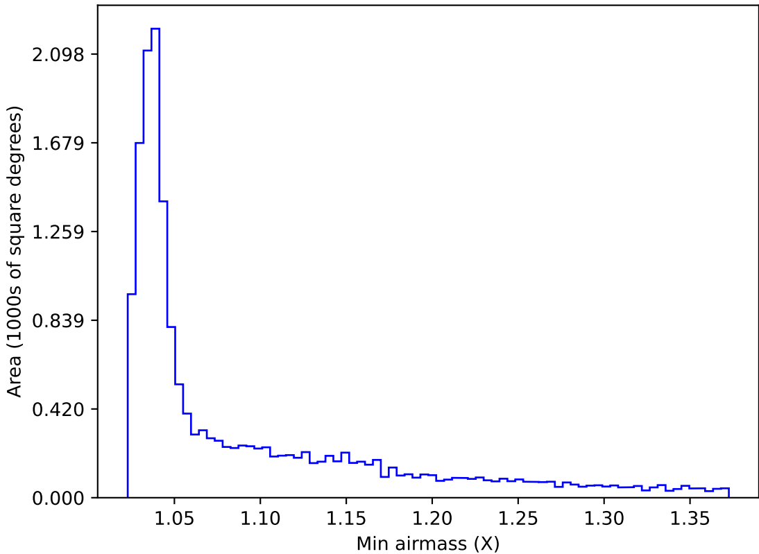
ddf_acor_sf25_lsf40_lsr20_v3.4_10yrs WFD g band: Min airmass
