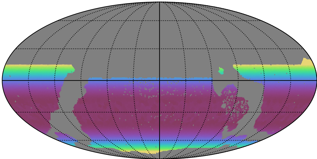
ddf_acor_sf25_lsf40_lsr20_v3.4_10yrs WFD all bands: Min airmass
