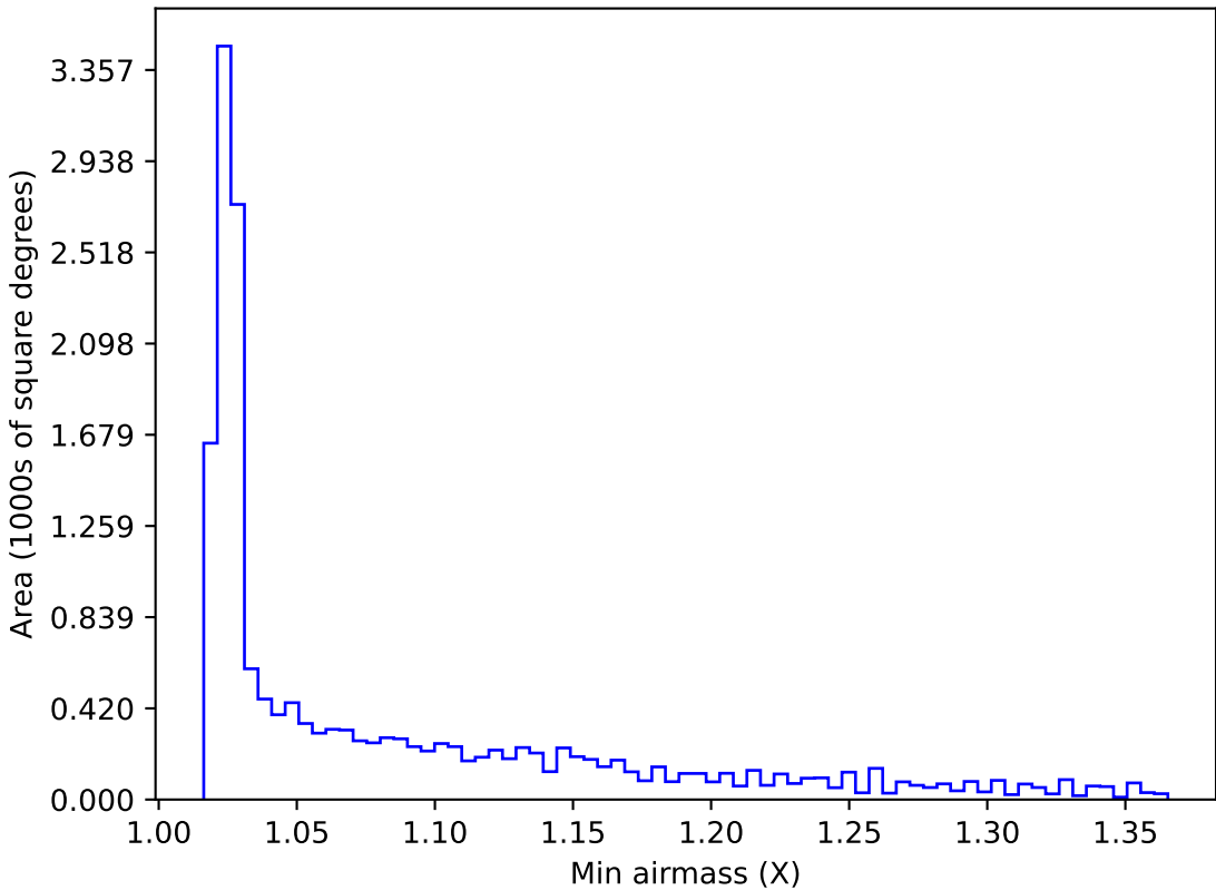
ddf_acor_sf25_lsf40_lsr20_v3.4_10yrs WFD all bands: Min airmass
