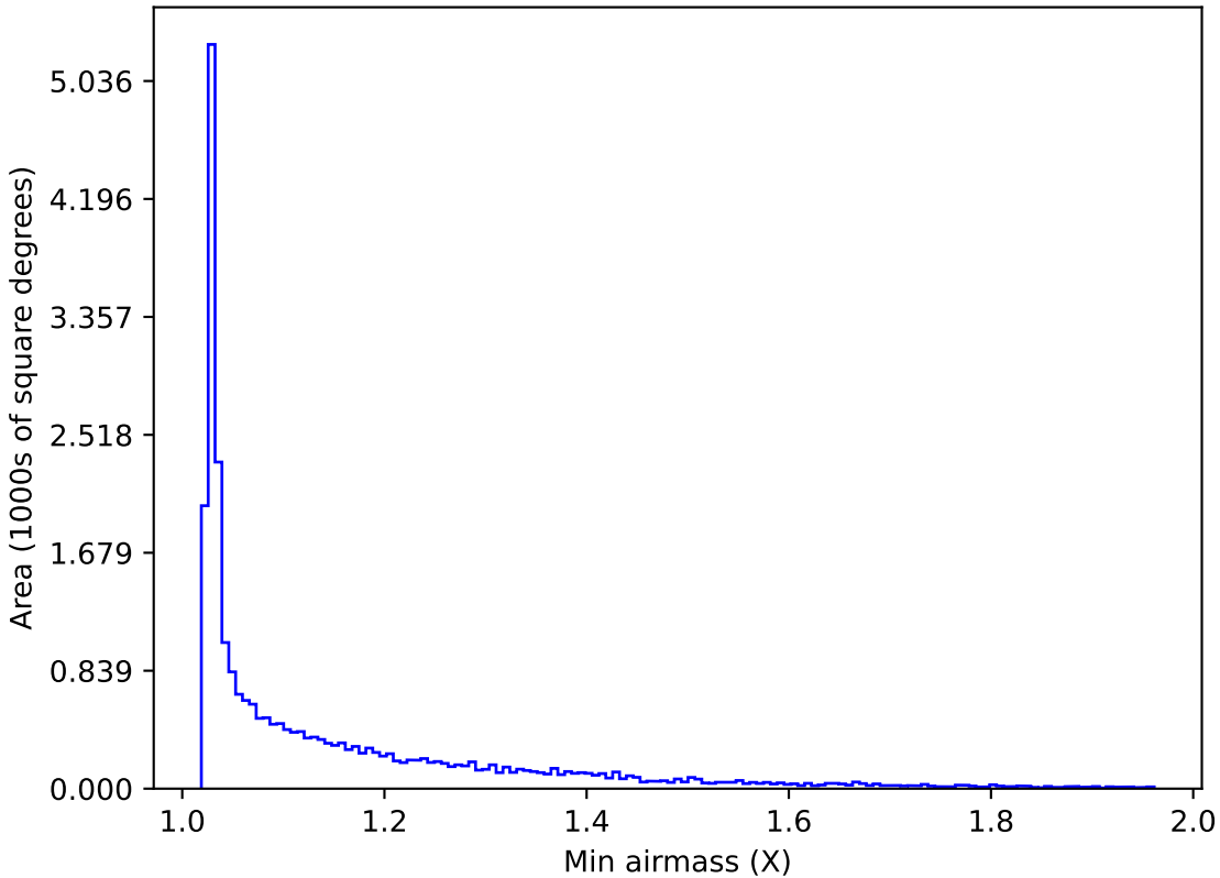
ddf_acor_sf25_lsf40_lsr20_v3.4_10yrs All sky z band: Min airmass
