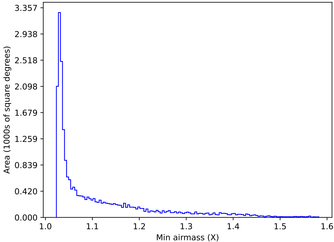
ddf_acor_sf25_lsf40_lsr20_v3.4_10yrs All sky y band: Min airmass
