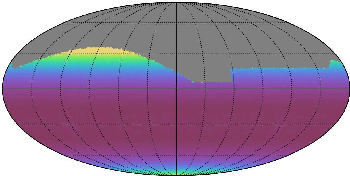
ddf_acor_sf25_lsf40_lsr20_v3.4_10yrs All sky r band: Min airmass
