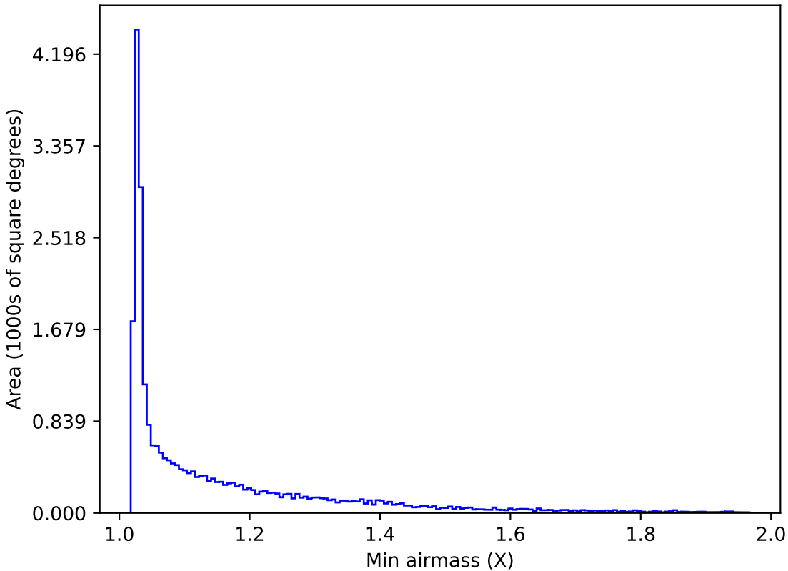
ddf_acor_sf25_lsf40_lsr20_v3.4_10yrs All sky r band: Min airmass
