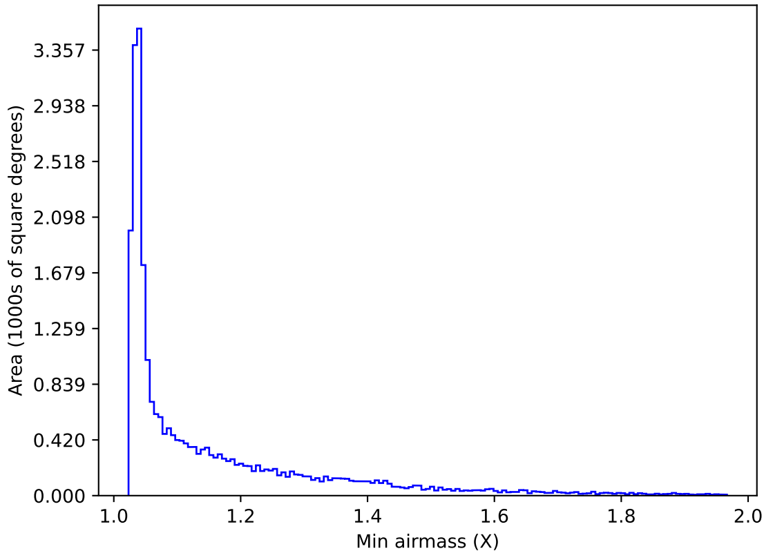
ddf_acor_sf25_lsf40_lsr20_v3.4_10yrs All sky g band: Min airmass
